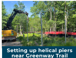
Installation of helical piers
